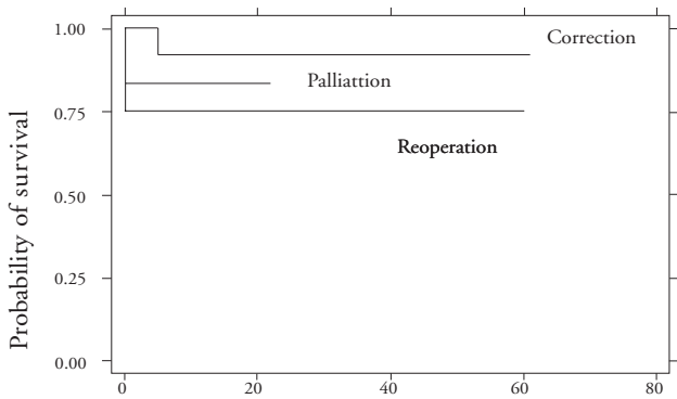
Figure 2. Kaplan-Meier survival function by type of surgery (palliatives , corrections, reoperation). Survival in 60 months probability in total correction type is 92.31% with 95% confidence bands (0.57-0.99), in reoperation type is 75% with 95% confidence bands (0.13-0.96) and in palliation type is 83.33% with 95% confidence bands (0.27-0.97)
